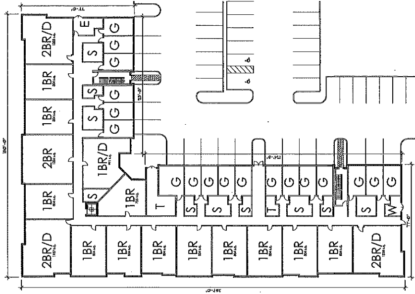
GROUND FLOOR PLAN SCALE 1/16" = 1'-0"
