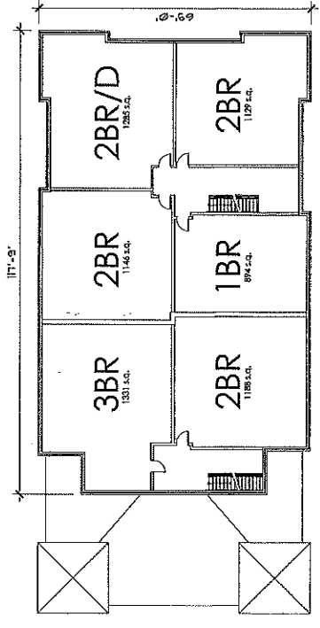
THIRD FLOOR PLAN SCALE 3/32" = 1'-0"
