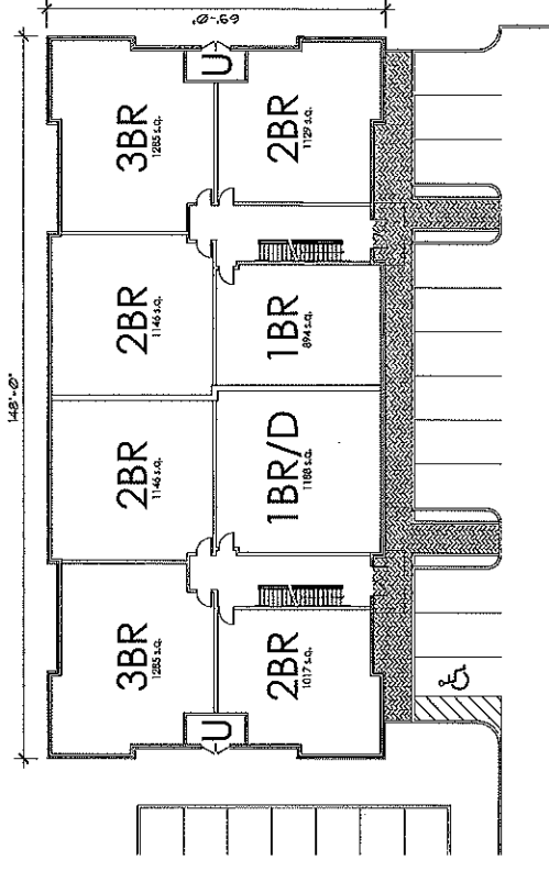
GROUND FLOOR PLAN SCALE 3/32" = 1'-0"
