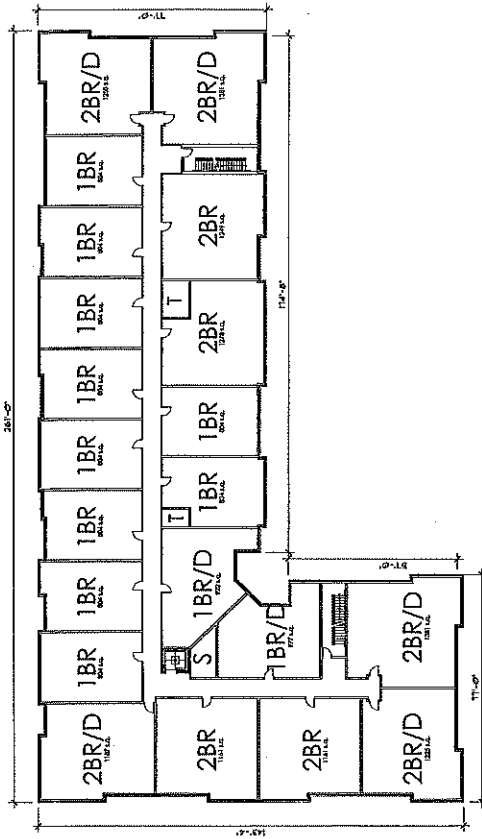
SECOND FLOOR PLAN SCALE 1/8" = 1'-0"
