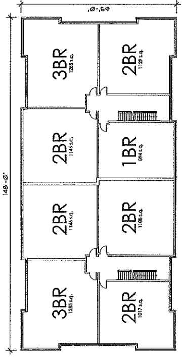
SECOND FLOOR PLAN SCALE 3/32" = 1'-0"
