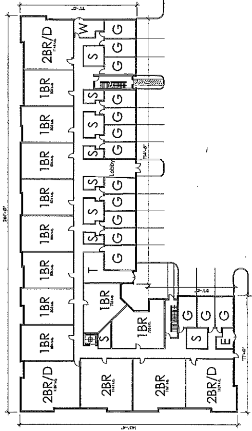
GROUND FLOOR PLAN SCALE 1/8" = 1'-0"
